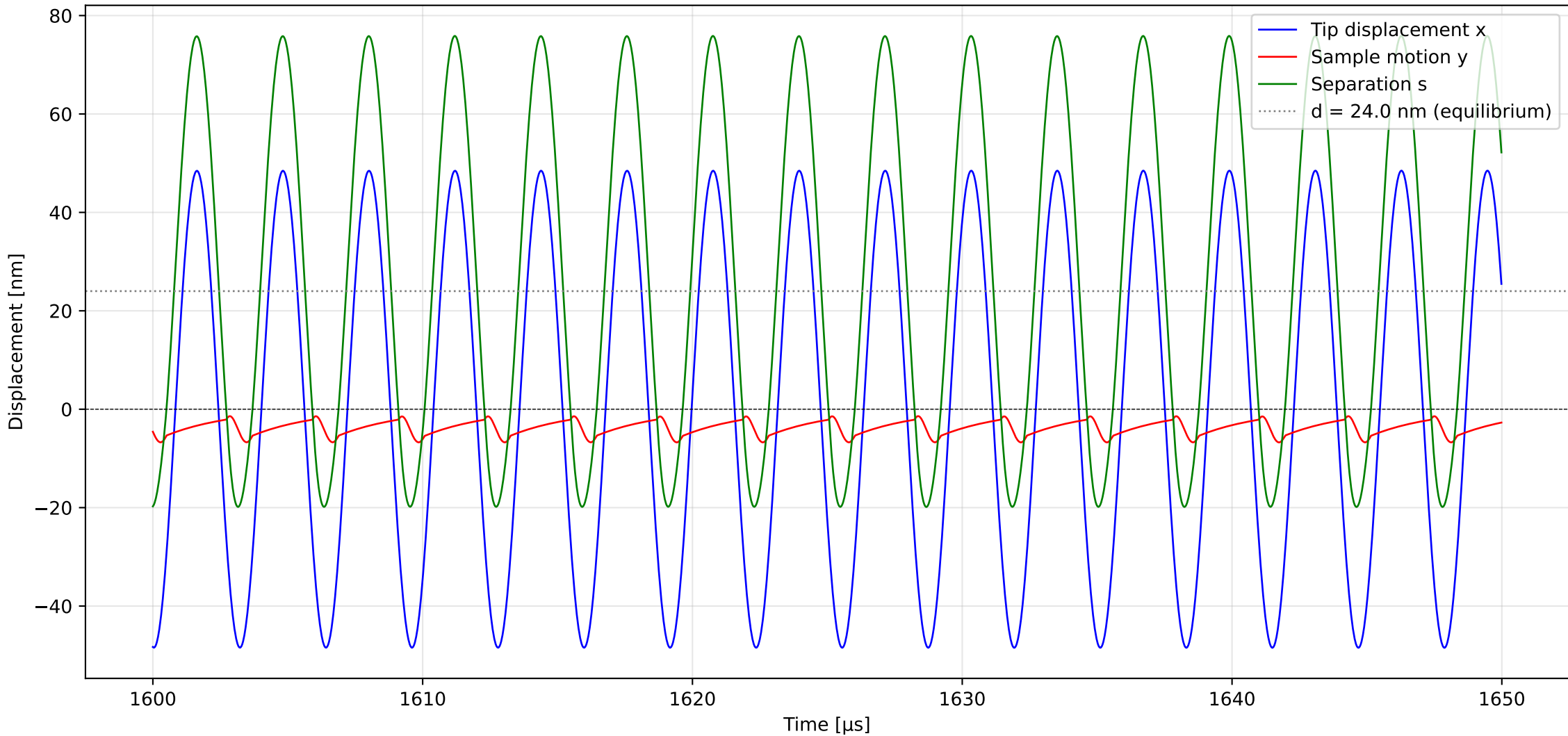
AFM DMT-KV: Tip, Sample, and Separation (1600-1650 \mu\text{s} , Steady-State)
